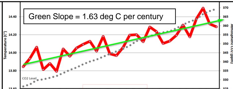
Warming During Large Human CO2 Emissions. 1970 to 2000 with 13.2% rise in CO2
