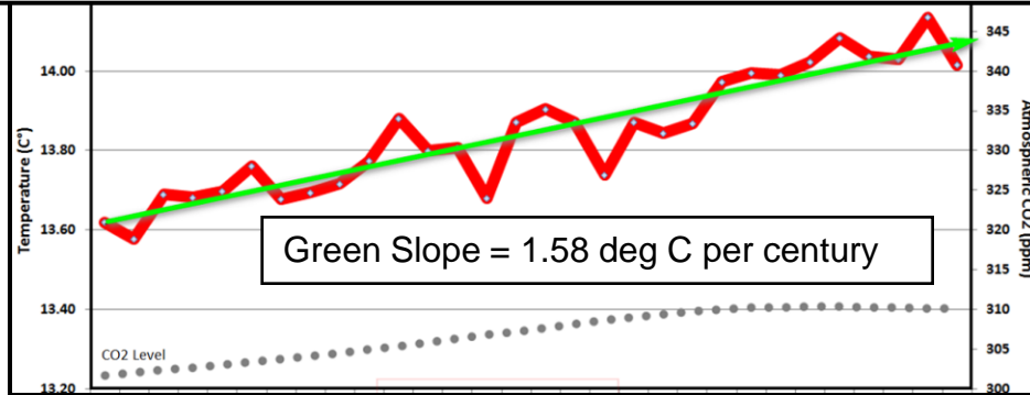
Warming Prior to Large Human CO2 Emissions. 1915 to 1945 with 2.7% rise in CO2
