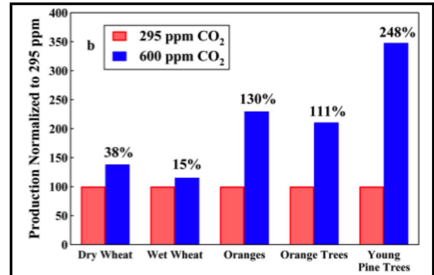
Figure 24: Calculated (1,2) growth rate enhancement of wheat, young orange trees, and very young pine trees already taking place as a result of atmospheric enrichment by CO 2 from 1885 to 2007 (a), and expected as a result of atmospheric enrichment by CO 2 to a level of 600 ppm (b).
