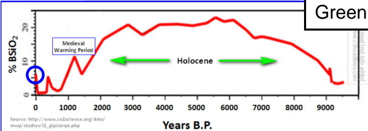
Past Global Warming Higher Temperatures From Lake In Greenland
