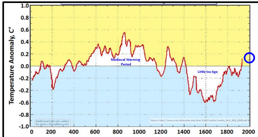
Last 2,000 years from 18 non-tree ring proxies (Dr Craig Loehle).
