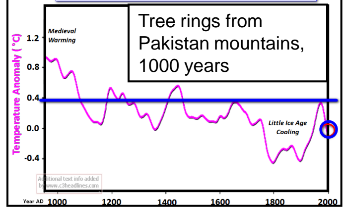
N. Pakistan Mountains Warmer During Medieval Period Summer Temps Higher With Less CO2
