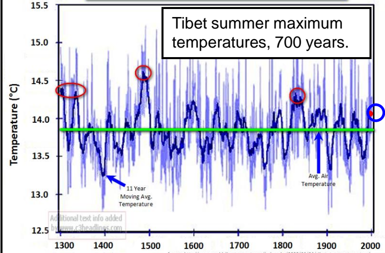
Little Ice Age Summer Temperatures In Tibet Maximum Temps Higher Than Modern Summers
